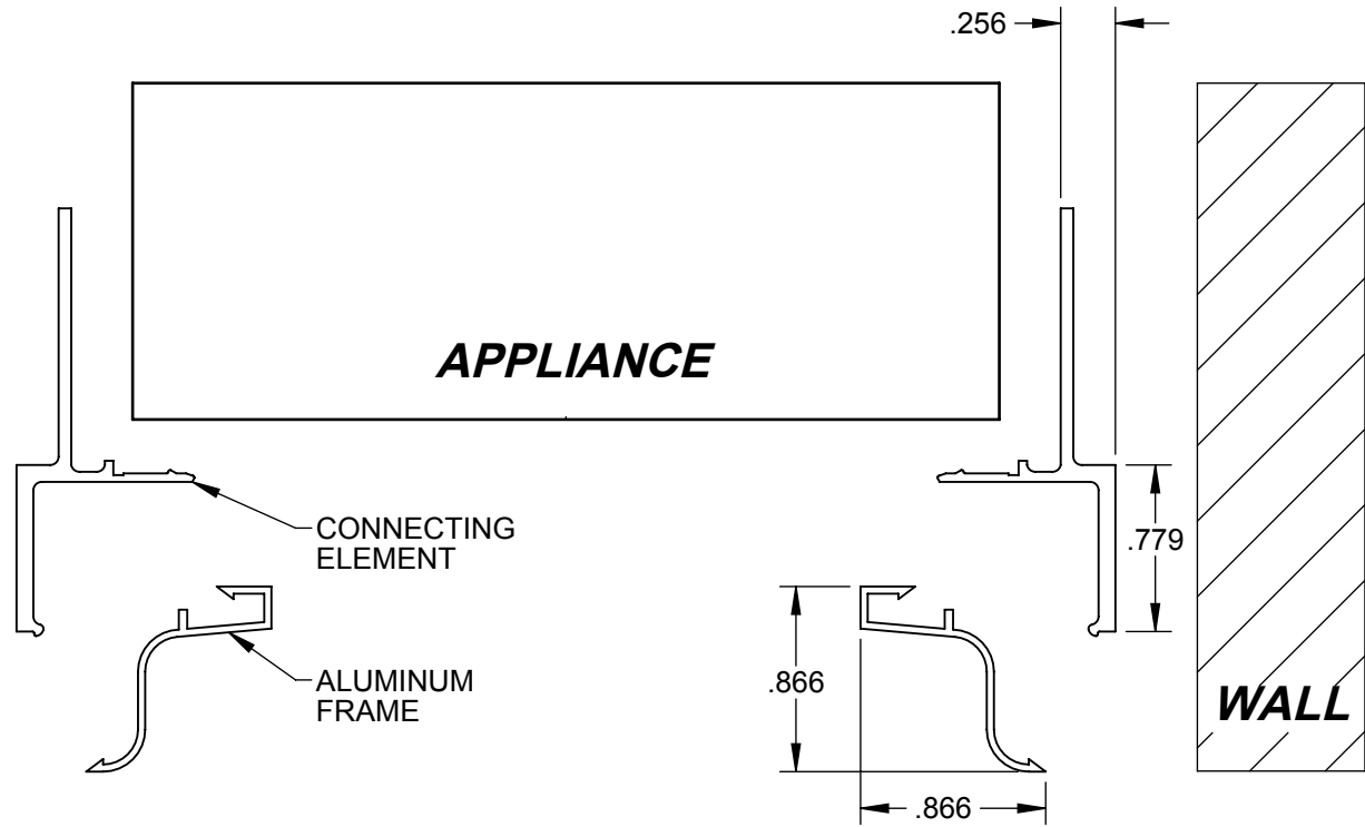
CROSS-SECTION VIEW
